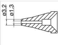
N60-03 Nozzle Size \Phi 1.3
