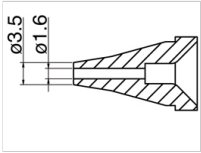
N60-04 Nozzle Size \Phi 1.6
