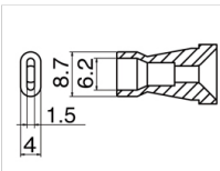
N60-09 Nozzle Size 6.2 x 1.5
