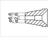
N60-06 Nozzle Size \Phi 2.6
