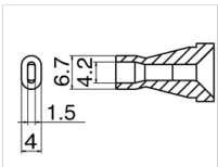
N60-08 Nozzle Size 4.2 x 1.5
